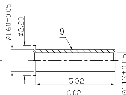
SCALE 4:1 CD013942022-4
