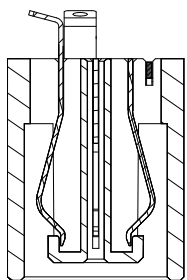
SECTION B-B
