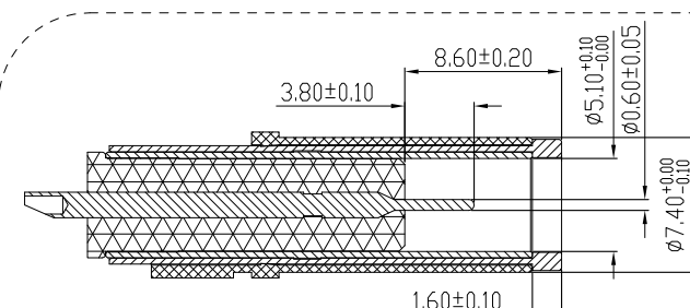
MATING PLUG
