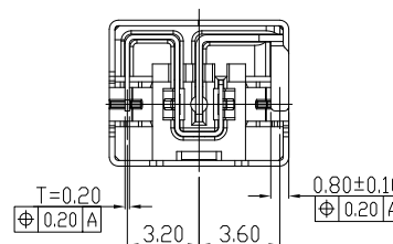
MATING PLUG
