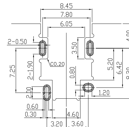
RECOMENDED PCB LAYOUT TOLERANCE:±0.05mm
