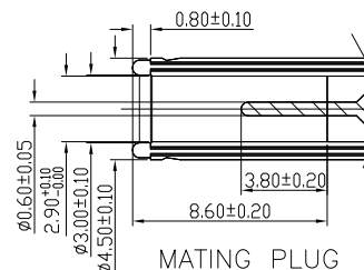
MATING PLUG
