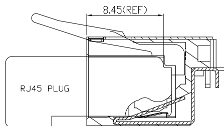
RJ45 PLUG MATED VIEW
