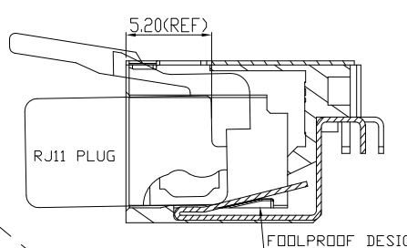
RJ11 PLUG MATED VIEW
