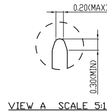
VIEW A SCALE 5:1
