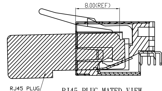
RJ45 PLUG MATED VIEW
