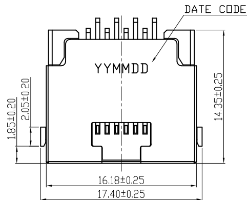
VIEW A SCALE 5:1
