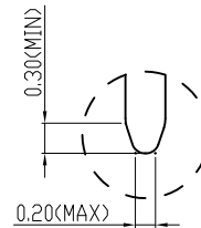
VIEW A SCALE 5:1
