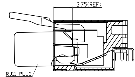
RJ11 PLUG MATED VIEW
